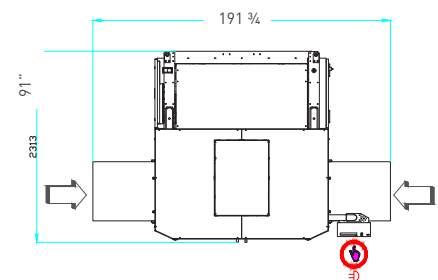
Machine height 192"
